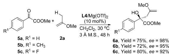
Scheme 3. Catalytic asymmetric hetero-ene reaction of \alpha -ketoesters.
